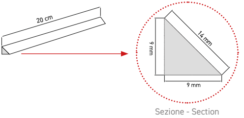
Dettaglio quarter round - Quarter round detail
