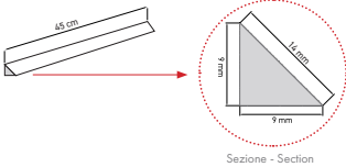
Dettaglio quarter round - Quarter round detail
