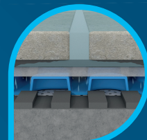
PRODESOS® DRAIN 8 SYSTEM
